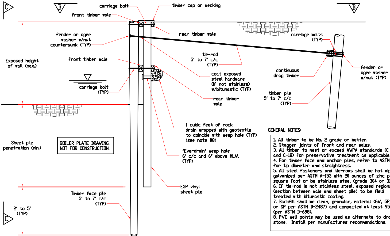
TYPICAL SECTION OF NAVY STYLE BULKHEAD (View A-A)
